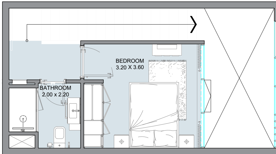
FIRST LEVEL
