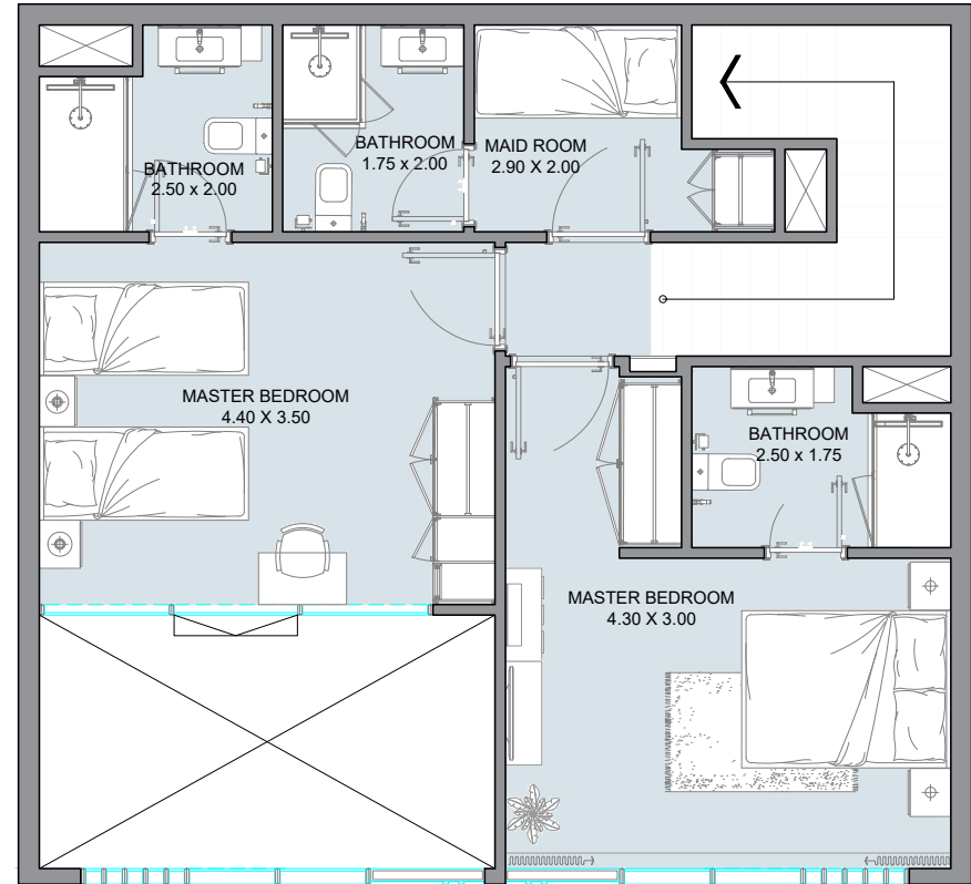
FIRST LEVEL
