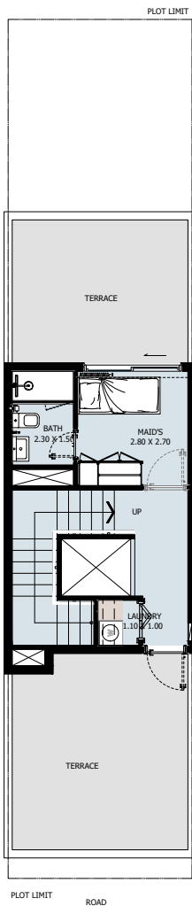
3RD FLOOR
