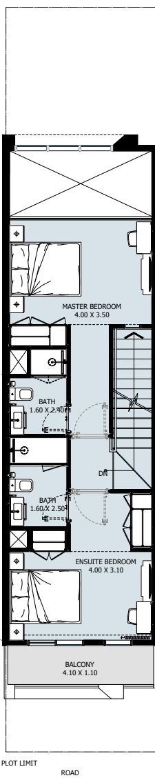
1ST FLOOR
